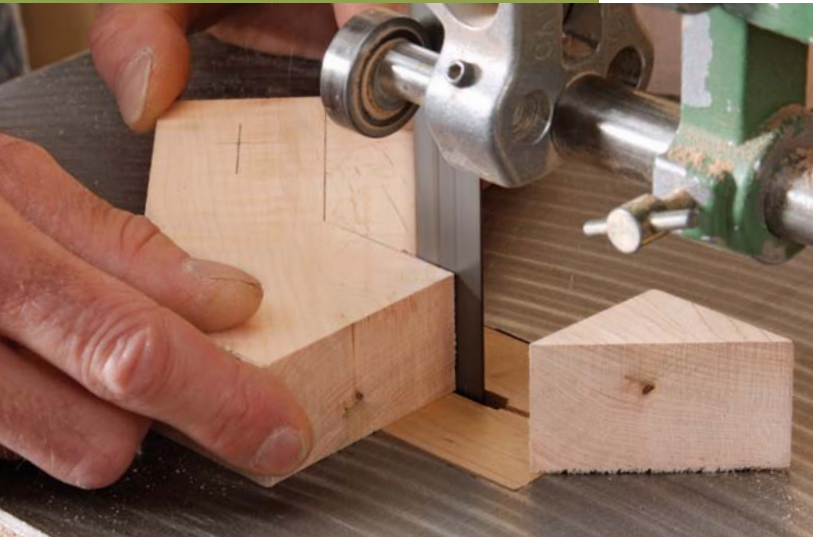
Cut the body to shape. All the cuts are easily made on the bandsaw. Make the angled cuts first (above), then use a fence to finish the straight inside cut (right).
